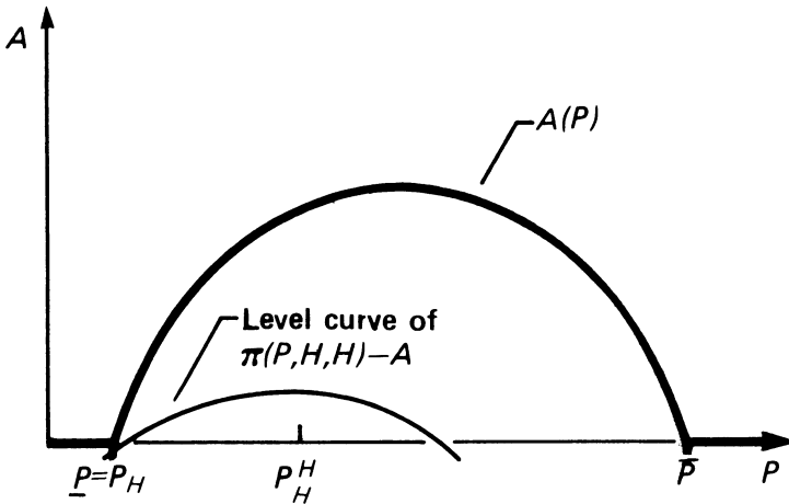
FIG. 4.—Condition (7) holds; equilibrium at (\bar{P}, 0)
