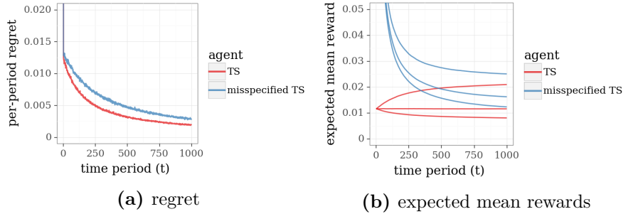
Figure 6.2: Comparison of TS for the Bernoulli bandit problem with coherent versus misspecified priors.
