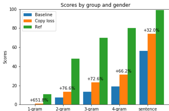
Figure 2: Plot shows percentage of novel [1,2,3,4]-grams in generated summaries from baseline model, our model and reference summary.
