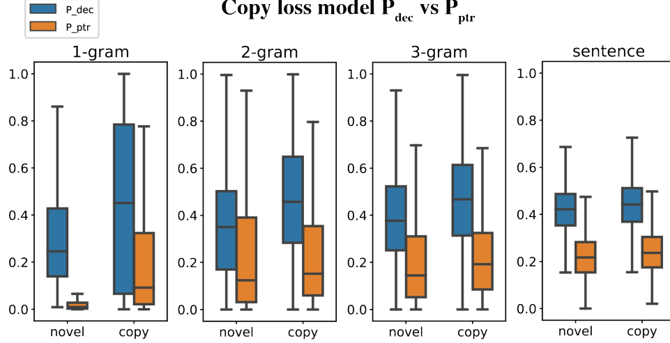
Figure 4: Comparison of P_{DEC} vs P_{PTR} for copy loss model [1,2,3]-gram and sentences.
