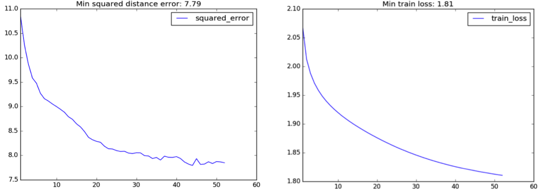
Figure 4: Train loss and squared loss vs. epochs for simple 2-hidden layer model used to classify 5-grams into buckets
