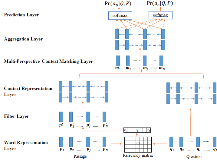
Figure 1. Architecture for Multi Perspective Context Matching Model. [1]
